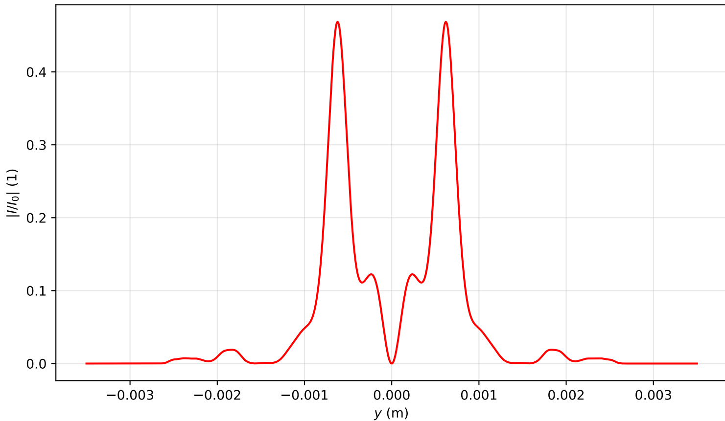
Intensity profile I(x=0, y, z=1.592)/I_0 , \text{Pin}=9.0\text{Pcr} , artificial time
